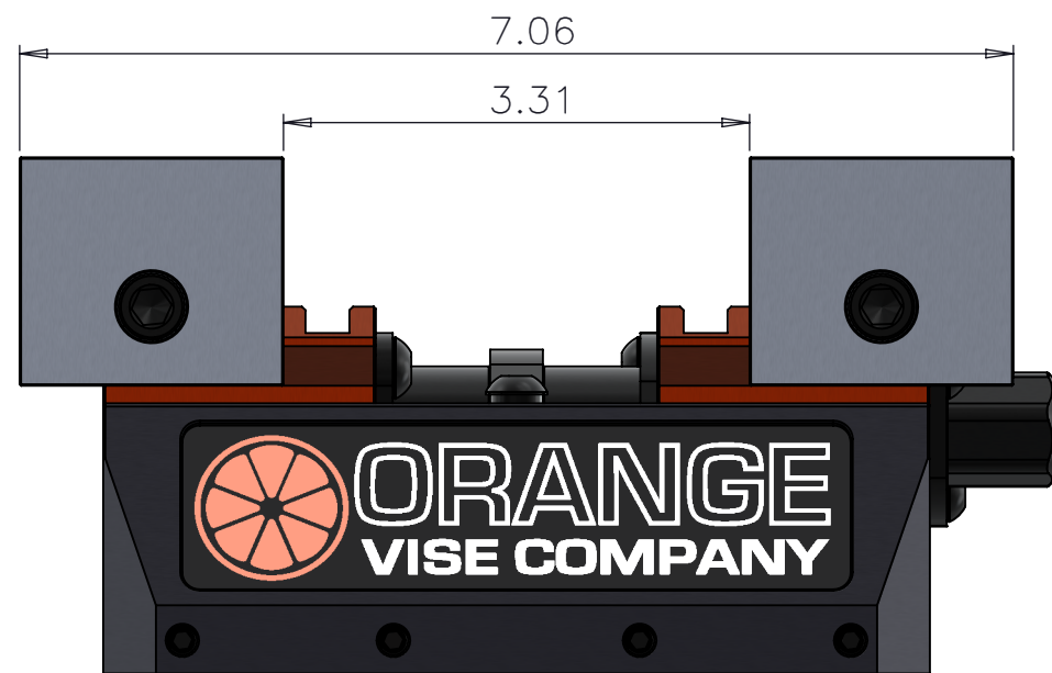
OUTBOARD JAW CONFIGURATION 1.25" JAW STROKE
