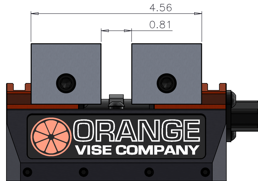
INBOARD JAW CONFIGURATION (OPENED) CLOSES TO ZERO
