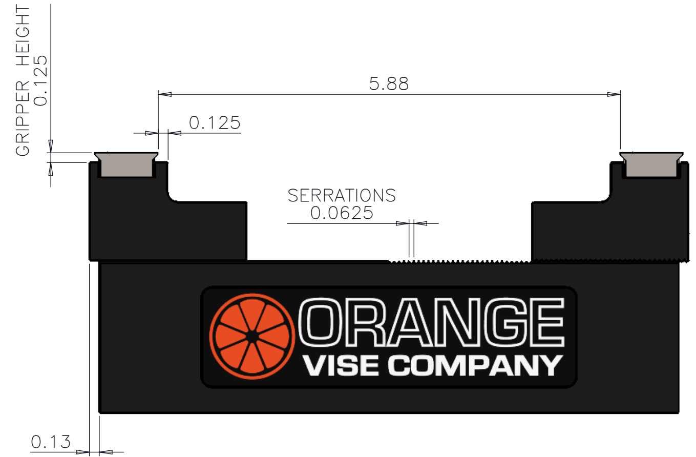
MASTER JAWSET B FULLY OPENED
