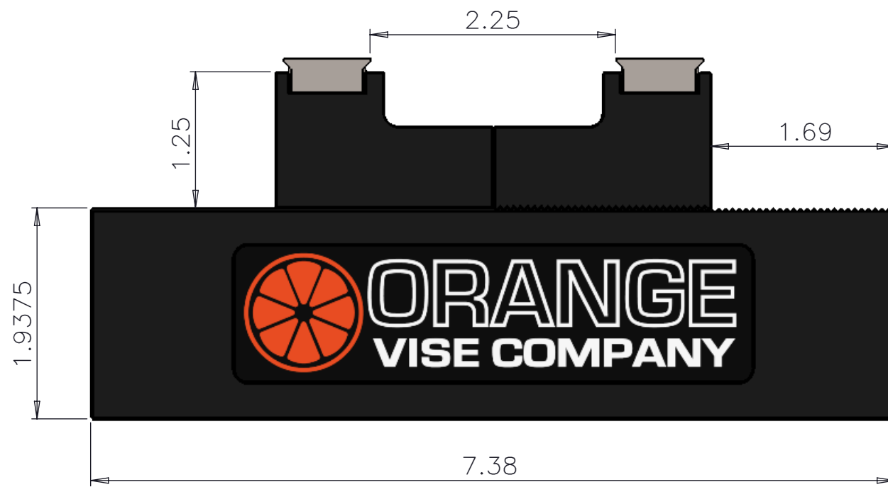
MASTER JAWSET B FULLY CLOSED
