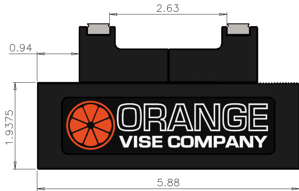
MASTER JAWSET B FULLY CLOSED
