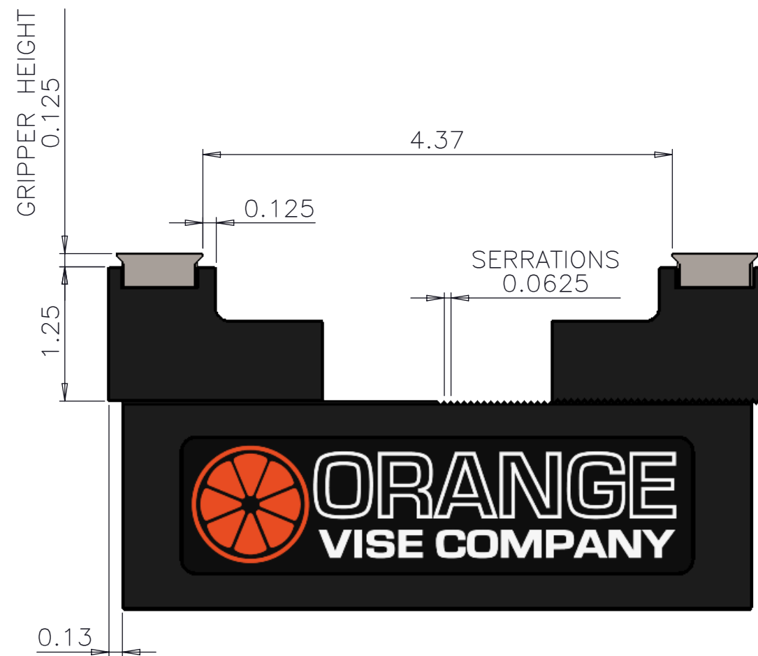
MASTER JAWSET B FULLY OPENED
